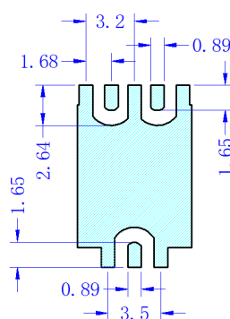
Suggested PCB Layout
